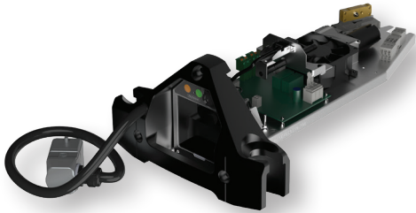
Aero 325 Retrofit Top Beam E-Tray
